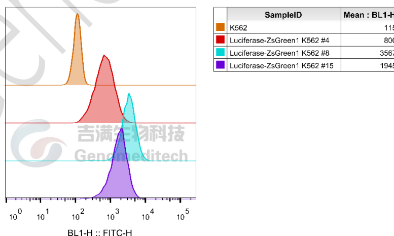
Figure 2 | Flow cytometry analysis of green fluorescent protein (GFP) expression in Luciferase-ZsGreen1 K562 Cell Line (Cat. GM-C24924).
